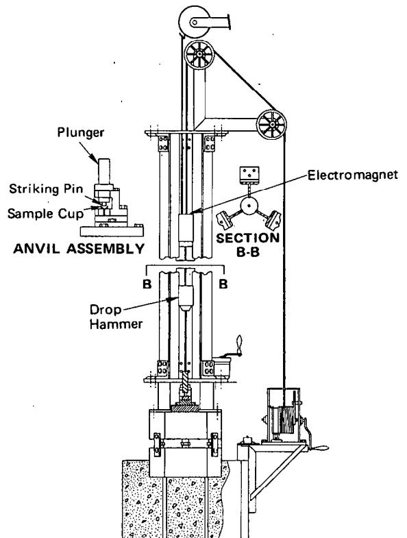
Fig 4. Impact Apparatus Showing Anvil-striking Pin Assembly
